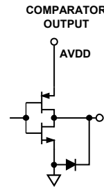
Figure 22. Comparator Outputs
